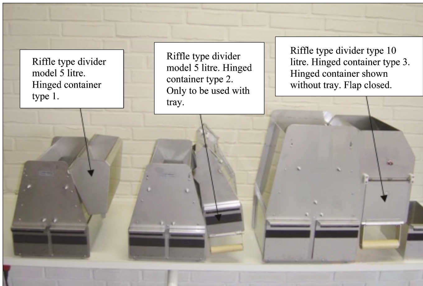
Riffle type dividers shown with different types of hinged containers
